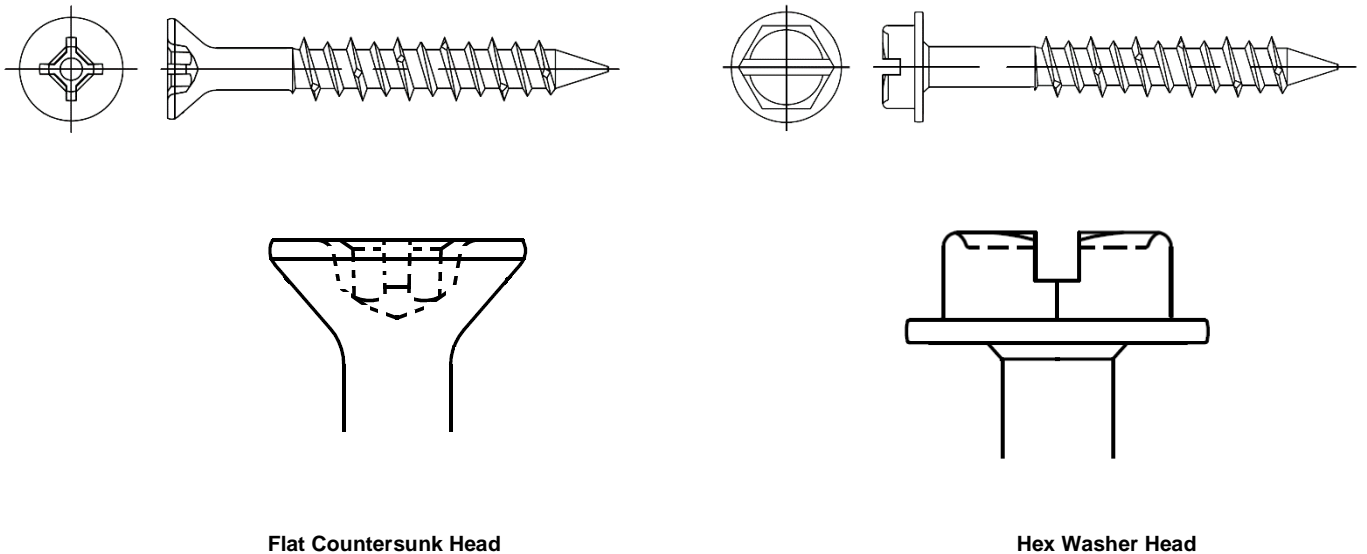
Flat Countersunk Head
